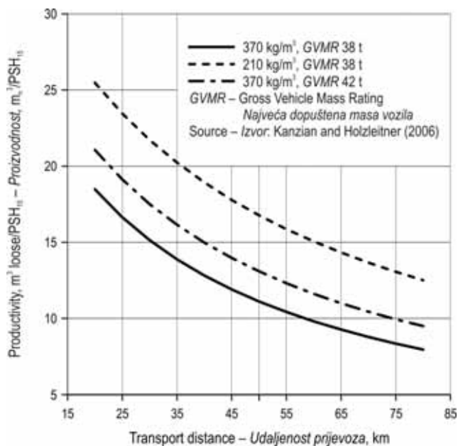
Fig. 8 Productivity in relation to the bulk density of the material transported and the maximum allowable total truck mass
