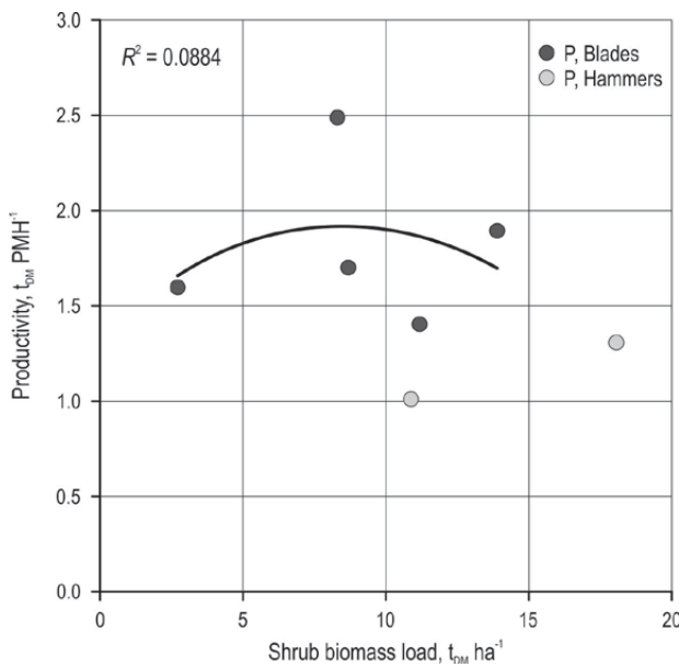
Fig. 4 Influence of standing shrub biomass load (BL, t_{DM} \cdot ha^{-1} ) on harvester-baler biomass productivity ( P , t_{DM} \cdot PMH^{-1} )
