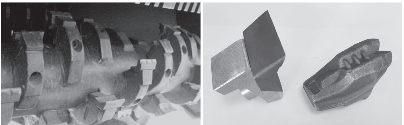
Fig. 3 (a) Harvester cutting rotor provided with blades; (b) Blade (left) and fix hammer (right)
