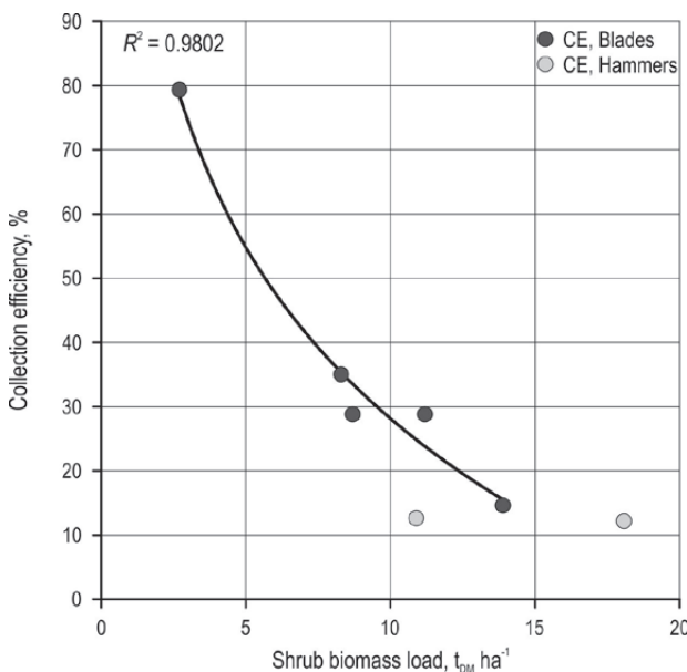
Fig. 5 Influence of standing shrub biomass load (BL, t_{DM} \cdot ha^{-1} ) on biomass collection efficiency (CE, %)
