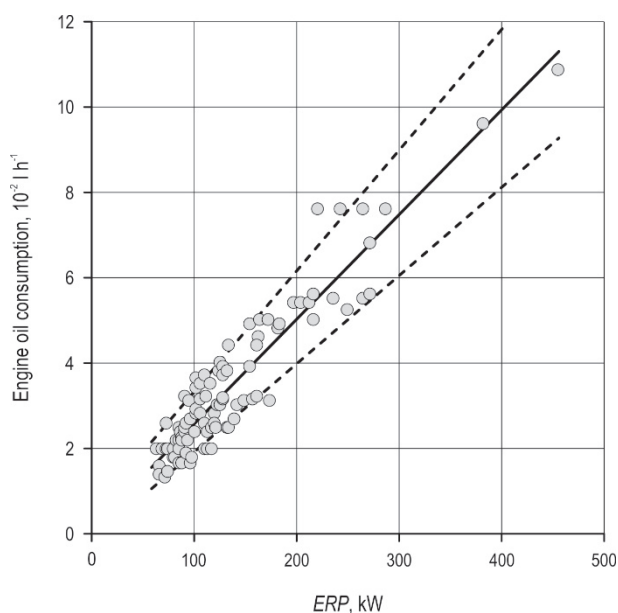
Fig. 2 Plot of engine oil consumption every 100 hours of machine work ( 10^{-2} \text{ l h}^{-1} ) as a function of engine rated power ERP (kW), regression line PEOCO and 95% confidence interval
