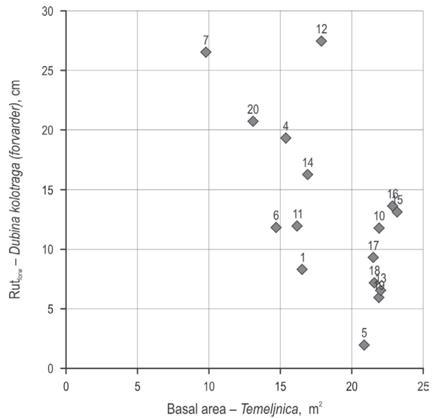
Fig. 7 Covariation between rut depth of forwarder and basal area Slika 7. Ovisnost dubine kolotruga forvardera i temeljnica
