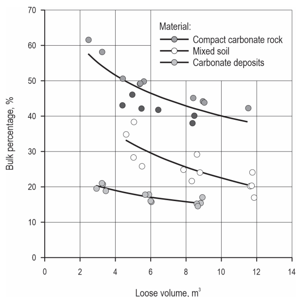
Fig. 5 Calculated bulk percentages for compact carbonate rock, mixed soil, and carbonate deposits; points for plots 5 and 6 (in black) indicate compact carbonate rock with greater porosity than in plots 1 to 4
